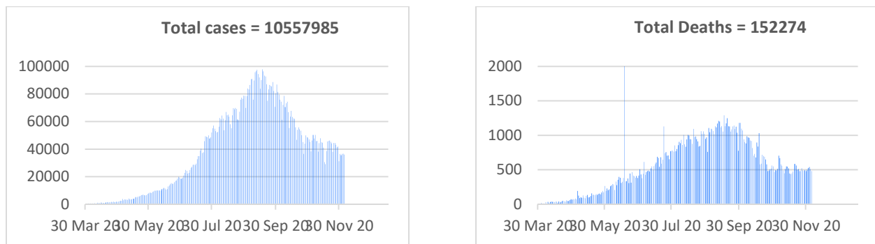
Fig.20: Left: Daily new cases; Right: Daily new deaths (till 16 th January, 2021).
