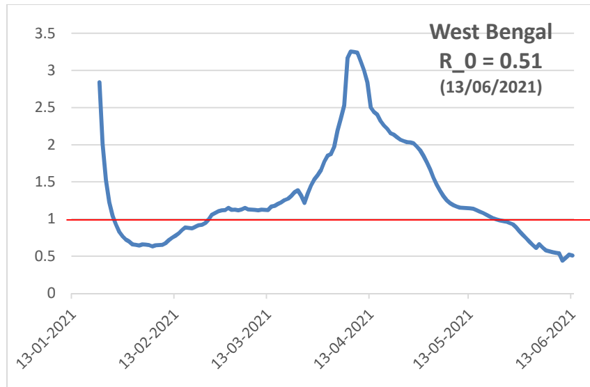
Fig. C: Evolution of basic reproduction rate ( R_0 ) with time (till 13 th June, 2021). The red horizontal line indicates R_0 = 1 .
