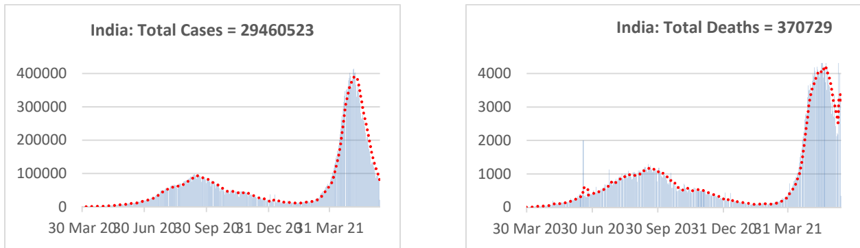
Fig. B: Left: Daily new cases; Right: Daily new deaths (till 13 th June, 2021). Red dotted lines show trend (5 days rolling average) of the curve.
