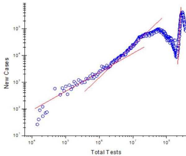
Fig.II: Daily new cases vs. total tests (till 11 th June, 2021). Red continuous lines are guide to eyes.
