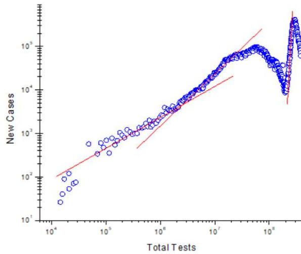
Fig.II: Daily new cases vs. total tests (till 14 th June, 2021). Red continuous lines are guide to eyes.
