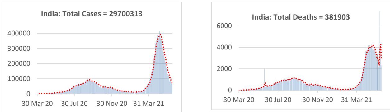
Fig. B: Left: Daily new cases; Right: Daily new deaths (till 16 th June, 2021). Red dotted lines show trend (5 days rolling average) of the curve.
