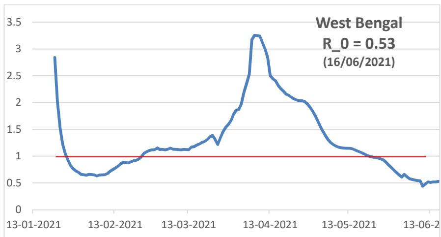
Fig. C: Evolution of basic reproduction rate ( R_0 ) with time (till 16 th June, 2021). The red horizontal line indicates R_0 = 1 .
