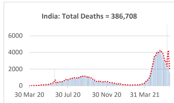
Fig. B: Left: Daily new cases; Right: Daily new deaths (till 19 th June, 2021). Red dotted lines show trend (5 days rolling average) of the curve.
