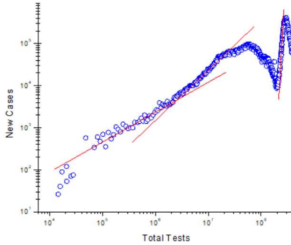
Fig.II: Daily new cases vs. total tests (till 17 th June, 2021). Red continuous lines are guide to eyes.
