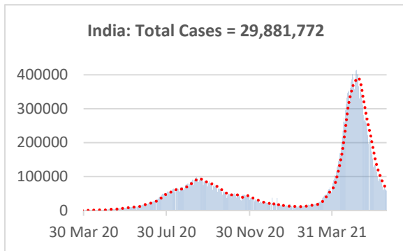
Fig. B: Left: Daily new cases; Right: Daily new deaths (till 19 th June, 2021). Red dotted lines show trend (5 days rolling average) of the curve.
