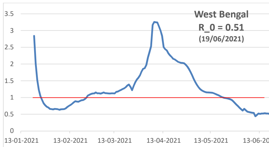
Fig. C: Evolution of basic reproduction rate ( R_0 ) with time (till 19 th June, 2021). The red horizontal line indicates R_0 = 1 .
