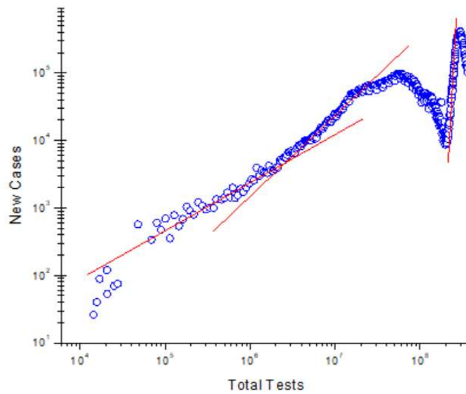
Fig.II: Daily new cases vs. total tests (till 6 th June, 2021). Red continuous lines are guide to eyes.
