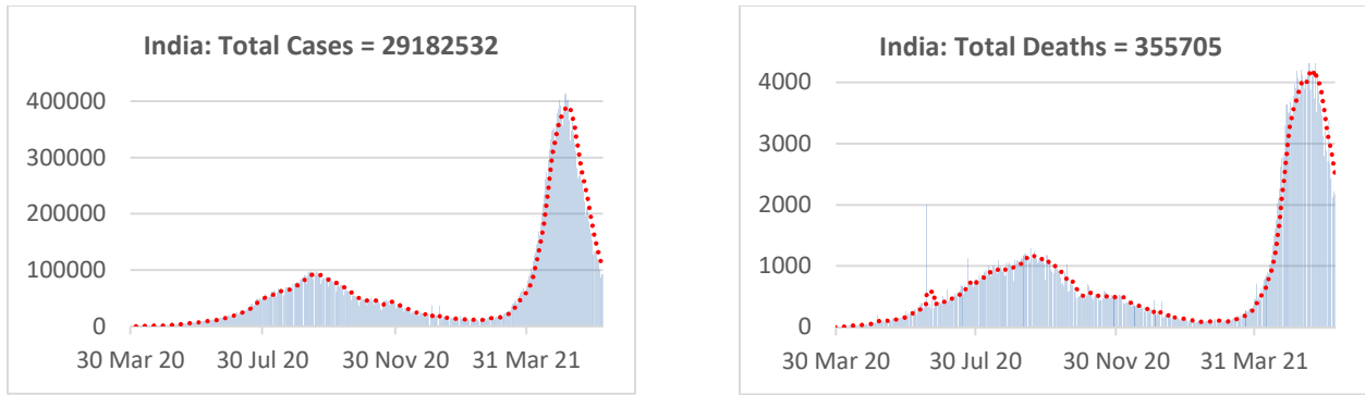
Fig. B: Left: Daily new cases; Right: Daily new deaths (till 9 th June, 2021). Red dotted lines show trend (5 days rolling average) of the curve.
