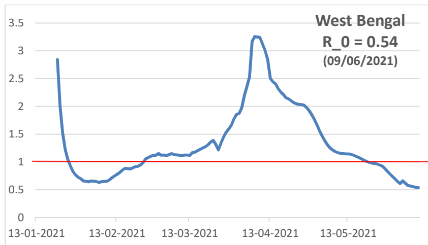
Fig. C: Evolution of basic reproduction rate ( R_0 ) with time (till 9 th June, 2021). The red horizontal line indicates R_0 = 1 .
