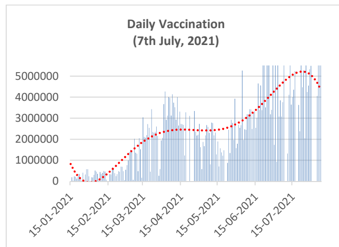
Fig.VII: Daily vaccination. Red dotted line shows trends of the curve.
