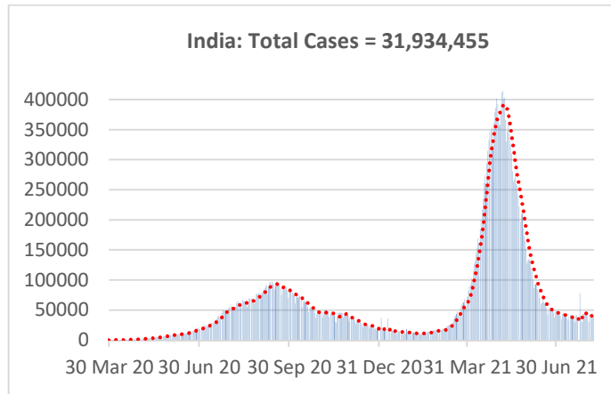
Fig. B: Daily new cases (last updated on 7 th August, 2021). Red dotted line shows trend (5 days rolling average) of the curve.
