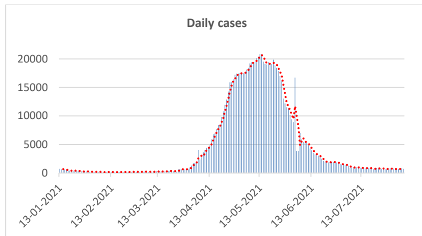
Fig. E: (For West Bengal) Daily new cases . Red dotted lines show trend (3 days rolling average) of the curve.
