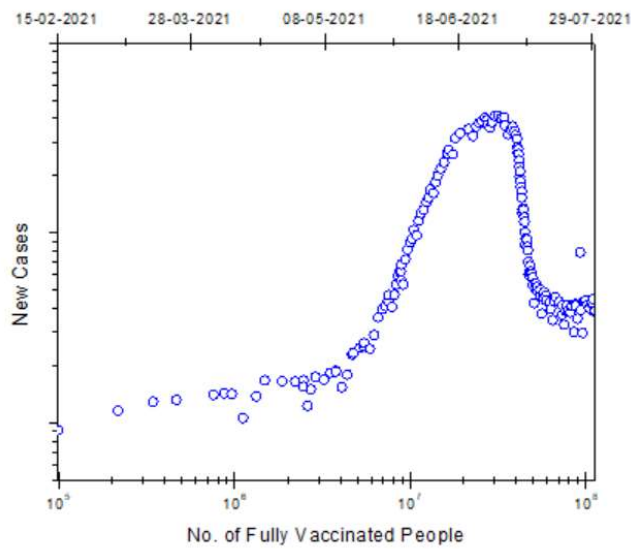
Fig.IV: Daily new cases with respect to number of fully vaccinated population (last updated on 30 th July, 2021).
