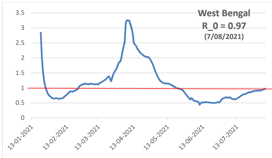
Fig. D: Evolution of basic reproduction rate ( R_0 ) with time. The red horizontal line indicates R_0 = 1 .
