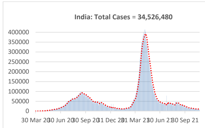
Fig. B: Daily new cases (last updated on 22 nd November, 2021). Red dotted line shows trend (5 days rolling average) of the curve.
