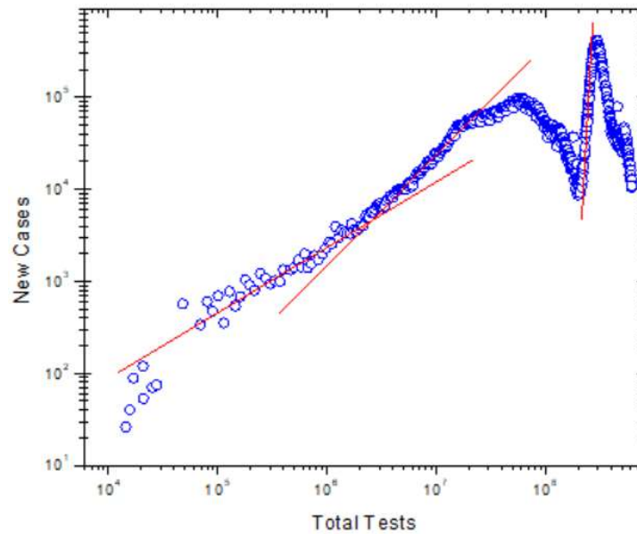
Fig.II: Daily new cases vs. total tests. Red continuous lines are guide to eyes (last updated on 22 nd November, 2021).
